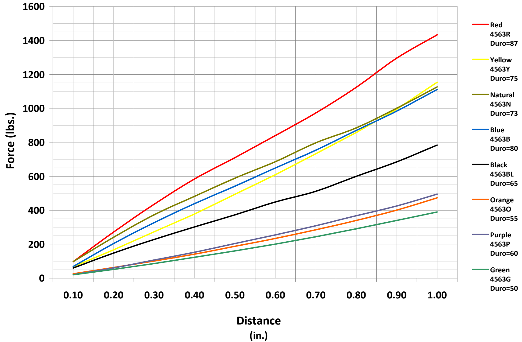
4563 Three Bushing Compression Graph
